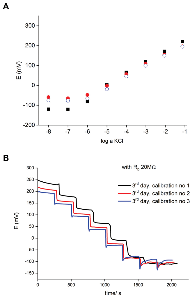
Fig. 4 (A) Selected potentiometric calibration plots for potassium-selective ISE, bypassed by zinc wire and resistor R_b = 20 \text{ M}\Omega , third calibration for each consecutive day is presented: (■) 1st day, (●) 2nd day (○) 3rd day. (B) Time traces for the sequential calibrations of the 3rd day.
