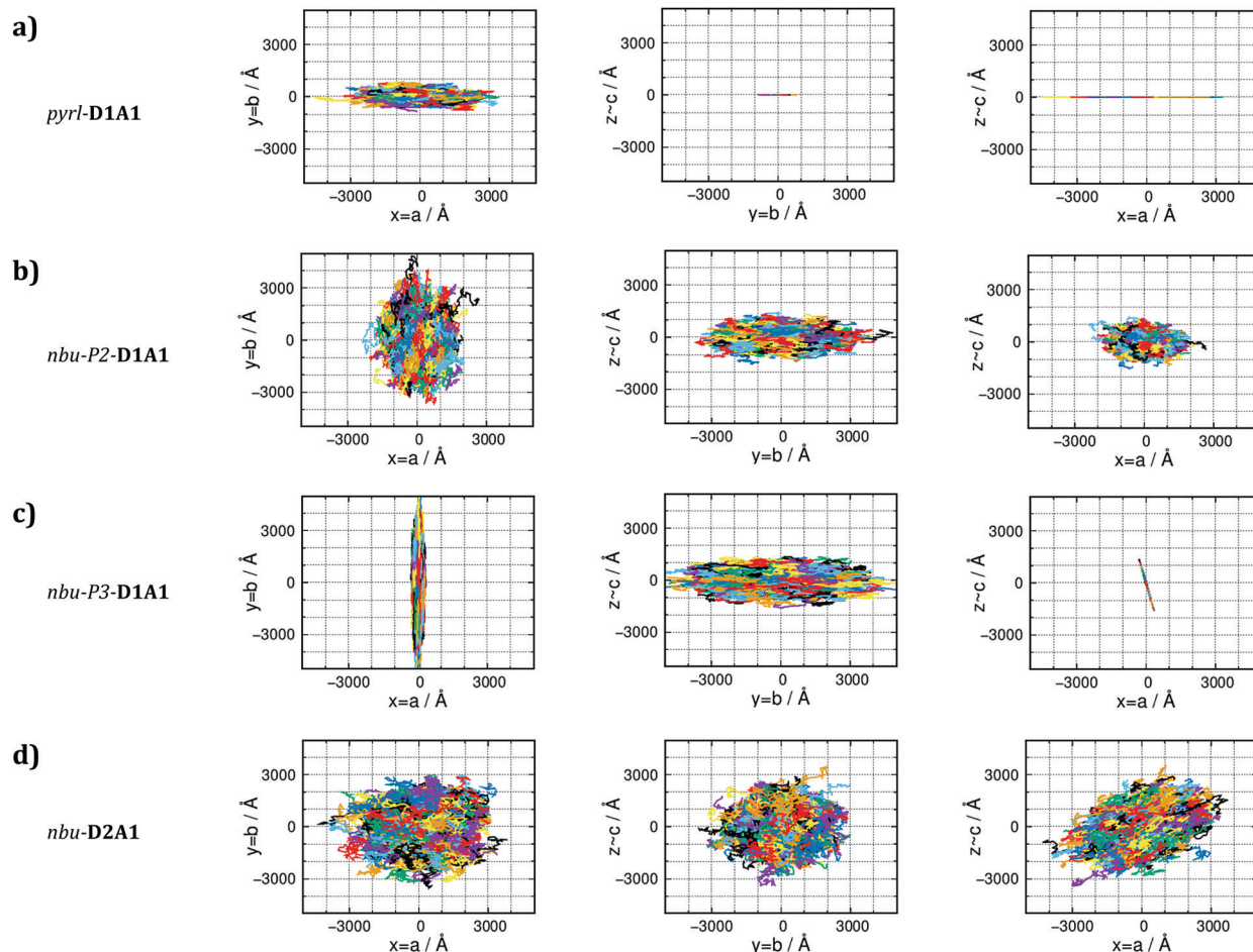
Fig. 7 Plot of 1000 kMC trajectories (each consisting of 10^5 steps) for each D1A1 and D2A1 class (from top to bottom: pyr1 -, nbu-P2 -, nbu-P3 - D1A1 and nbu-D2A1 ). Trajectories are reported for the three Cartesian planes, namely yx , zy and zx (crystallographic axes are reported as well).
