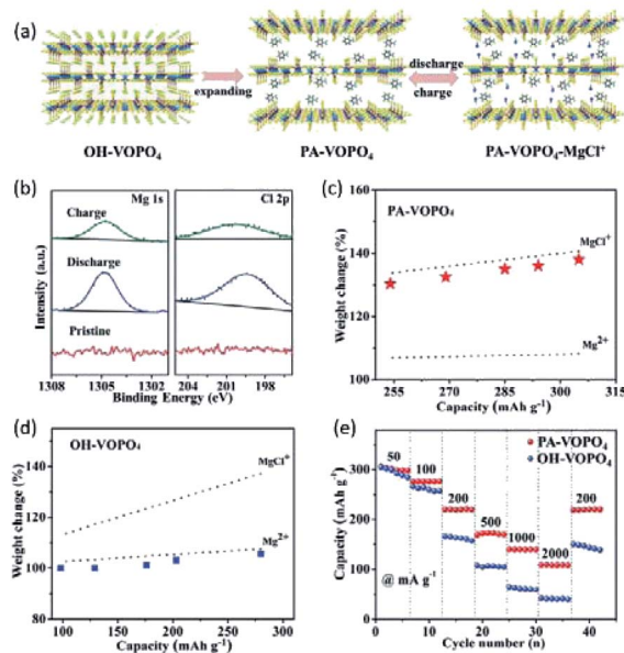
Fig. 14 (a) Schematic illustration of the experimental approach and proposed mechanism of PA-VOPO 4 nanosheets as the Mg-storage material. (b) Mg 1s and Cl 2p XPS spectra of PA-VOPO 4 nanosheets at the fully charged/discharged states. Mass change of the electrodes upon discharge when (c) PA-VOPO 4 nanosheets and (d) VOPO 4 ·2H 2 O bulk served as cathode materials. (e) Rate capability of VOPO 4 ·2H 2 O bulk and PA-VOPO 4 nanosheets. Reprinted with permission from ref. 153. Copyright 2018 Wiley-VCH Verlag GmbH & Co. KGaA, Weinheim.
