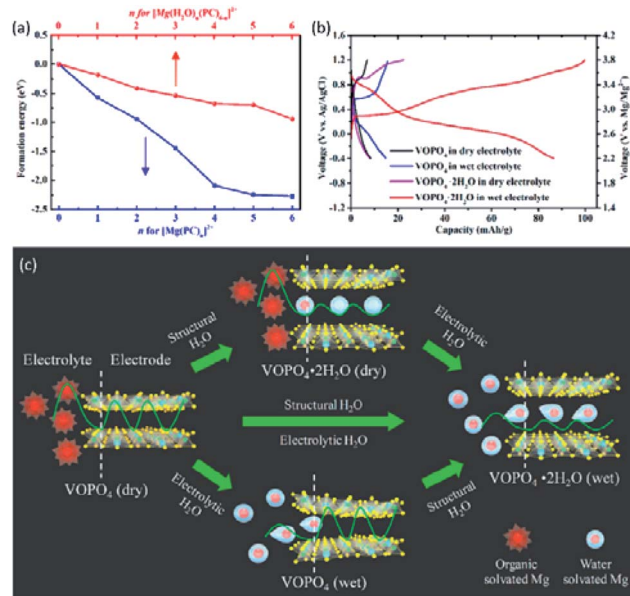
Fig. 13 (a) Formation energies of [Mg(PC) n (H 2 O) 6-n ] 2+ ( n \leq 6 ). (b) Voltage profiles of VOPO 4 and VOPO 4 ·2H 2 O in the water-free (0.1 M Mg(ClO 4 ) 2 in PC) and water-containing (0.1 M Mg(ClO 4 ) 2 ·6H 2 O in PC) electrolytes at 5 mA g -1 in a three-electrode cell with Ag/AgCl and active carbon as the reference and counter electrode, respectively. (c) Schematic illustrating the charge storage mechanism of VOPO 4 ·nH 2 O in the water-free and water-containing electrolytes. The green curves indicate the activation energy barriers, and the white dash lines represent the electrode/electrolyte interface. Reprinted with permission from ref. 152. Copyright 2018 American Chemical Society.
