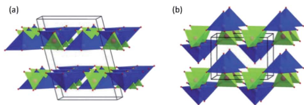
Fig. 11 Representation of (a) the \alpha_1 - \text{VOPO}_4 structure ( C2/m , a = 8.73187(14) Å, b = 6.20548(5) Å, c = 6.20902(4) Å and \beta = 104.448(3)^\circ at 280^\circ\text{C} ) and (b) the \alpha_2 - \text{VOPO}_4 structure ( P4/n , a = 6.0156(3) Å, c = 4.4375(3) Å at RT). Reproduced from ref. 147 with permission from The Royal Society of Chemistry.
