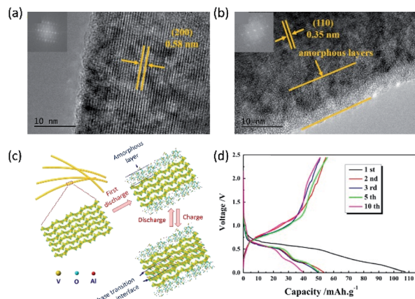
Fig. 10 (a and b) HRTEM images of the \text{V}_2\text{O}_5 nanowire (a) before cycling, and (b) at the fully discharged state (insets: fast Fourier transform images). (c) Schematic diagram showing the electrochemical \text{Al}^{3+} insertion/extraction of crystallized \text{V}_2\text{O}_5 nanowires. (d) Galvanostatic charge/discharge profiles of the \text{V}_2\text{O}_5 nanowire cathode. Reprinted with permission from ref. 108. Copyright 2017 Elsevier.
