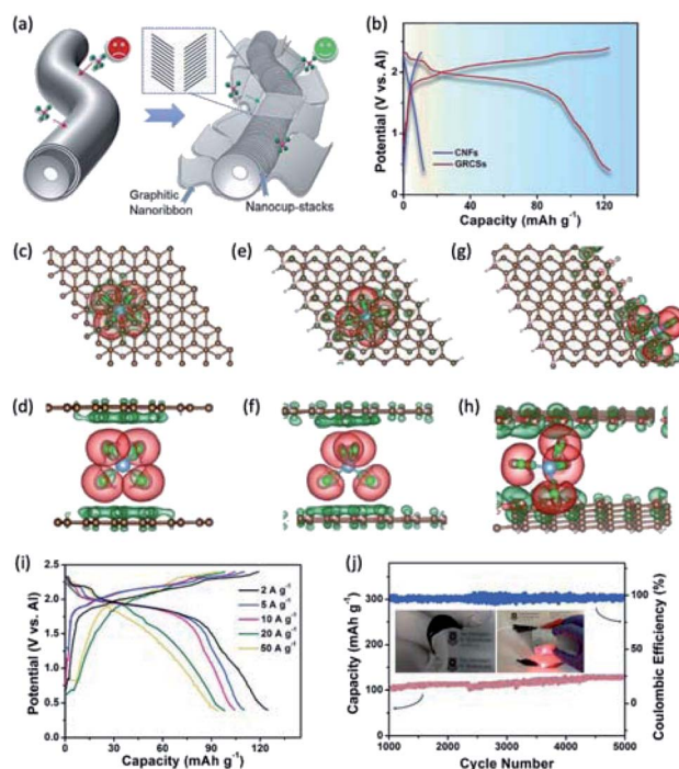
Fig. 26 (a) Schematic comparison of anion intercalation/deintercalation in commercial CNFs and cleaved CNFs. (b) Representative charge/discharge curves of CNFs and cleaved CNFs. (c–h) Calculated charge density differences of the \text{AlCl}_4^- in different graphene structures: the (c) top and (d) side views of the bilayer edge-less graphene with one \text{AlCl}_4^- ion placed between the two layers; the (e) top and (f) side views of the bilayer edge-rich graphene with one \text{AlCl}_4^- ion placed in the middle area; and the (g) top and (h) side views of bilayer edge-rich graphene with one \text{AlCl}_4^- ion placed near the edge, between two layers. An isosurface level of 0.0007 \text{ e}\text{\AA}^{-3} has been used in all images. (i) Charge/discharge curves of cleaved-CNFs at current densities from 2 to 50 \text{ A g}^{-1} . (j) Long-term stability of cleaved-CNFs with coulombic efficiency and discharge specific capacity versus the cycle number at a current density of 10 \text{ A g}^{-1} . The inset in d shows a flexible cleaved-CNFs electrode and a flexible AIB lighting a light emitting diode. Reproduced from ref. 186 with permission from The Royal Society of Chemistry.
