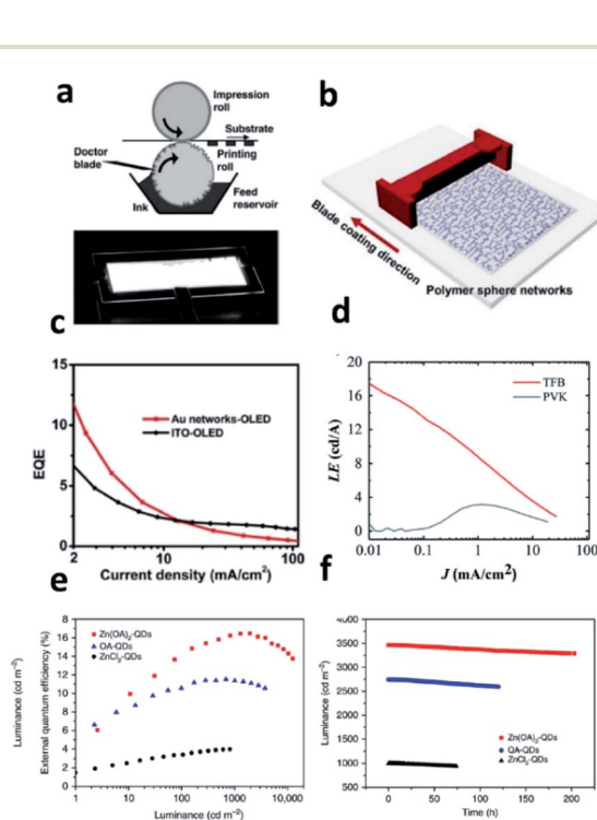
Fig. 4 (a) Schematic of large-scale OLED production via gravure printing; reproduced from ref. 53 with permission from Elsevier. (b) Fabrication process of Au micromesh transparent electrodes via blade-coating. (c) Device performance (EQE- J ) of printed OLEDs; reproduced from ref. 54 with permission from American Chemical Society. (d) Inkjet-printed OLEDs (LE- J ); reproduced from ref. 55 with permission from the Royal Society of Chemistry. (e and f) EQE and life time of \text{Zn(OA)}_2 -QDs vs. OA-QDs vs. \text{ZnCl}_2 -QDs devices; reproduced from ref. 56 with permission from Springer Nature.
