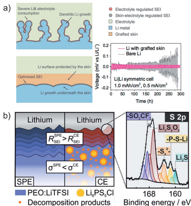
Fig. 16 (a) Schematic illustration of the formed protective surface layer and the voltage profile of a symmetric Li metal cell. Adapted with permission from ref. 194 CCC, copyright © 2017, American Chemical Society. (b) Schematic representation of the contribution of composite electrolyte decomposition products on SEI formation and corresponding X-ray photoelectron spectroscopy measurement of decomposition products observed in the S 2p signal. Adapted with permission from ref. 200 CCC, copyright © 2020, American Chemical Society.
