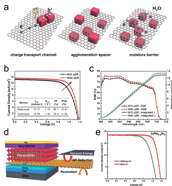
Fig. 9 Interfacial engineering of AIP QDs layers. (a) Schematic diagram of \mu\text{GR} 's effects on charge transport and stability under moisture for the \text{CsPbI}_3 film. (b) J-V curves and related parameters of the devices with and without \mu\text{GR} . (c) EQEs and the integrated products of the EQE curve with AM1.5G photon flux. Adapted with permission from ref. 104 Copyright 2018, Wiley-VCH. (d) Device structure with the modification of the interface by LiF. (e) J-V characteristics of inorganic \text{CsPbI}_{3-x}\text{Br}_x SCs with and without the LiF interlayer. Adapted with permission from ref. 124 Copyright 2019, Wiley-VCH.
