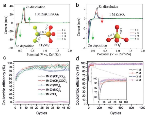
Fig. 8 (a) CV curves of Zn stripping/plating in 1 M Zn(CF 3 SO 3 ) 2 . (b) CV curves of Zn stripping/plating in 1 M ZnSO 4 . Reproduced with permission. 96 Copyright 2016, American Chemical Society. (c) Coulombic efficiency of Zn stripping/plating in different Zn salt electrolytes. (d) Coulombic efficiency of Zn stripping/plating in the Zn(CF 3 SO 3 ) 2 electrolyte with different concentrations. Reproduced with permission. 84 Copyright 2019, Wiley-VCH.
