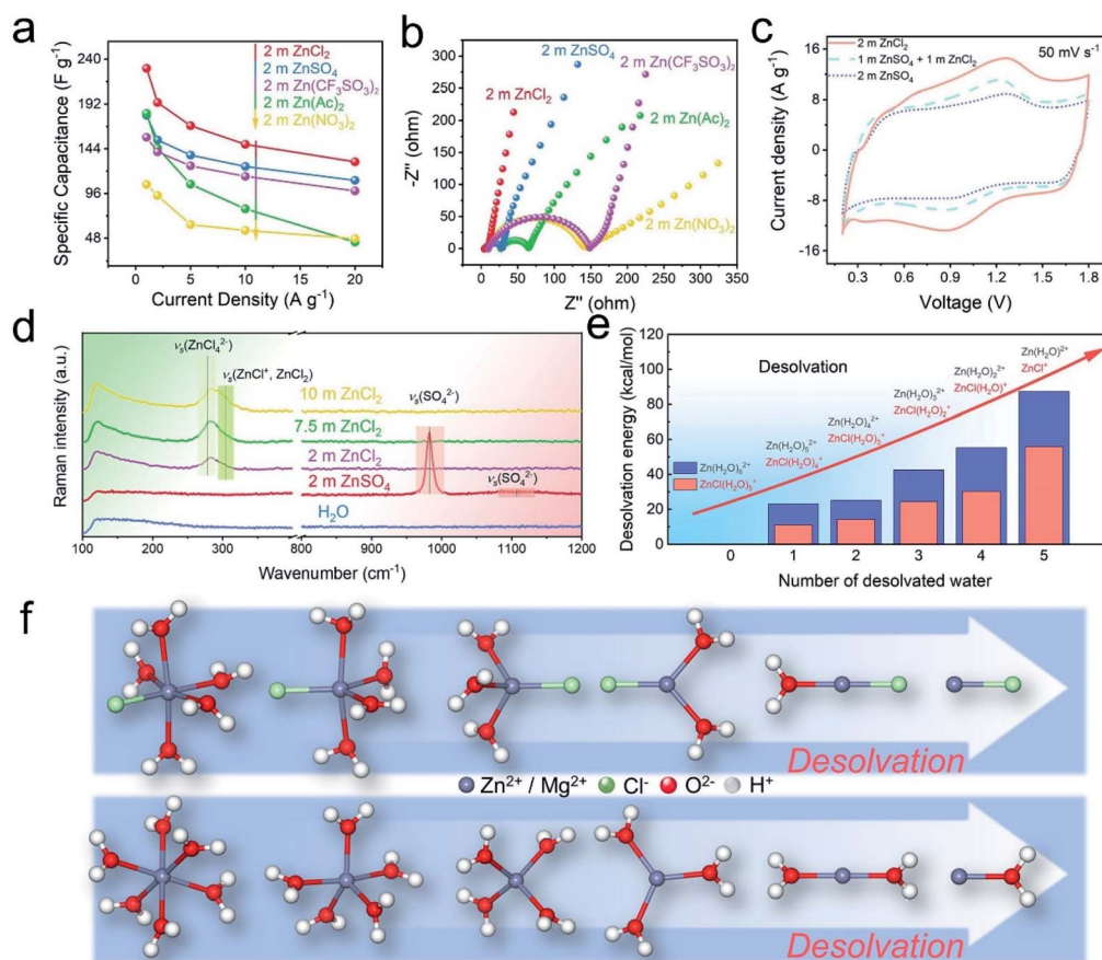
Fig. 9 (a) Rate capability of ZIHs in different zinc salt solutions. (b) Nyquist curves. (c) CV curves of ZIHs at 50 mV s -1 . (d) Raman spectra of different solutions. (e) Desolvation energies of [ZnCl(H 2 O) 5 ] + and [Zn(H 2 O) 6 ] 2+ . (f) Molecular geometries of the [ZnCl(H 2 O) 5 ] + and [Zn(H 2 O) 6 ] 2+ desolvation processes. Reproduced with permission. 58 Copyright 2020, Wiley-VCH.
