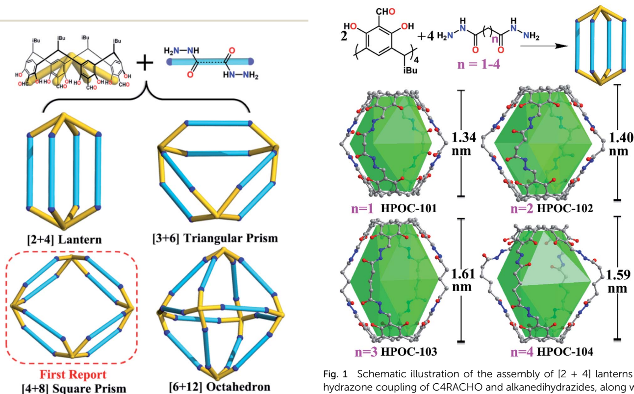
Scheme 1 Self-assembly of organic cages constructed from the tetraformyl C4RACHO cavitand and dihydrazide linkers.
