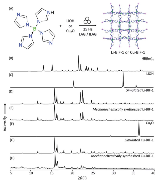
Fig. 3 (A) Reaction scheme for the mechanochemical synthesis of Li-BIF-1 using the acid–base strategy. Selected PXRD patterns for: (B) \text{H}[\text{B}(\text{Im})_4] (C) LiOH, (D) simulated Li-BIF-1 (CSD MOXJPEP), (E) synthesized BIF-1-Li by LAG for 60 minutes with MeCN ( \eta = 0.25 \mu\text{L mg}^{-1} ), (F) \text{Cu}_2\text{O} , (G) simulated Cu-BIF-1 (CSD MOXJIT), and (H) synthesized Cu-BIF-1 by ILAG for 60 minutes with MeOH ( \eta = 0.50 \mu\text{L mg}^{-1} ) and \text{NH}_4\text{NO}_3 additive (5% by weight).
