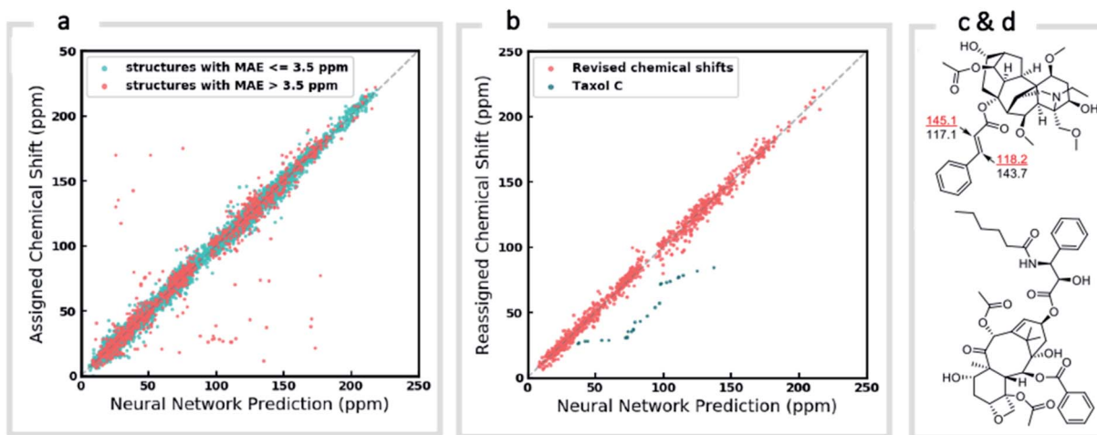
Fig. 6 Screening and revising misassignment in NMRShiftDB. (a) Correlation between predicted and experimental ^{13}\text{C} chemical shifts for large molecules ( \text{MW} > 500 ). Outliers (red), here defined as structures with an MAE > 3.5 ppm, are investigated for possible misassignments (b) experimental chemical shifts for reordered assignments of outlying structures. The remaining outliers (green) helped us to identify an incorrect structure for Taxol C in the database. (c) Incorrectly assigned enoate carbons were corrected for leueantine A. (d) The correct structure of Taxol C.
