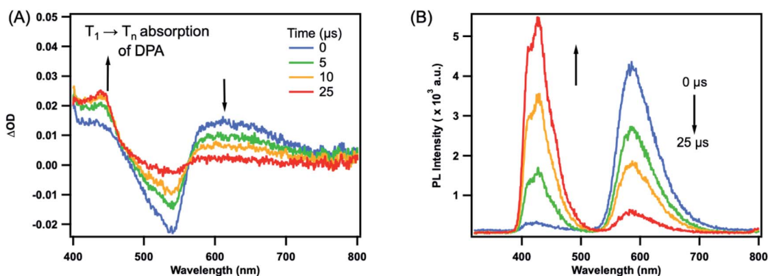
Fig. 3 Transient absorption difference spectra (A), and time-resolved photoluminescence spectra (B) of \text{Zr}(\text{MesPDP}^{\text{Ph}})_2 ( \text{OD}_{514 \text{ nm}} = 0.4 ) and 0.25 \text{ mM} DPA in deaerated THF at several delay times following 514 \text{ nm} pulsed laser excitation ( \sim 2 \text{ mJ} per pulse) with delay times indicated.
