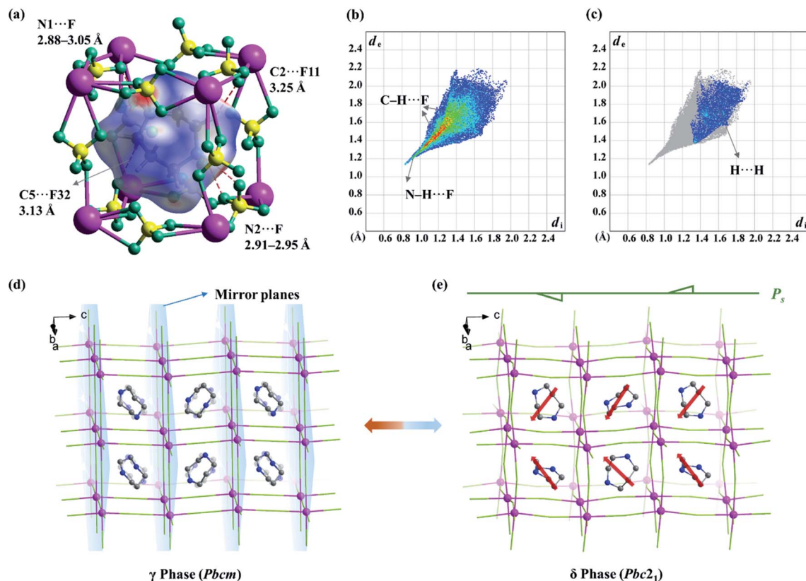
Fig. 7 (a) Hirshfeld surfaces mapped with d_{\text{norm}} over the range of -0.50 (red) to 0.90 (blue) for the guest cation at the \delta phase. Fingerprint plot for H \cdots F contacts (b) and H \cdots H contacts (c) of guest cations at the \delta phase. Crystal structures at 338 K ( \gamma phase, d) and 293 K ( \delta phase, e) along the diagonal of the (001) lattice plane. For clarity, H atoms are omitted. In the \gamma phase, the organic cations are located in two sites about the mirror planes (light blue planes). In the \delta phase, the orientations of ordered organic cations (the directions of dipole moment are shown in red arrows) induce spontaneous polarization along the c -axis and the disappearance of the mirrors in the \delta phase.
