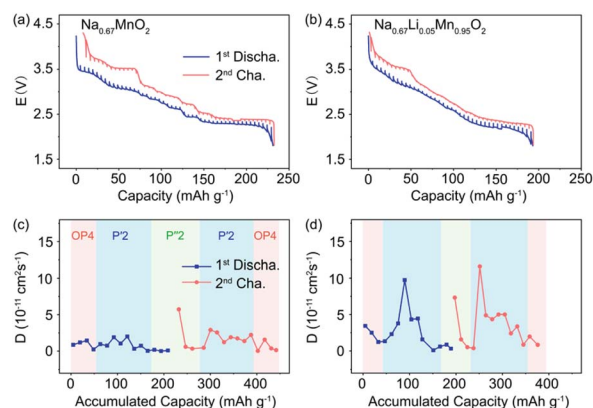
Fig. 5 GITT profiles of (a) P'2-Na 0.67 MnO 2 and (b) P'2-Na 0.67 Li 0.05 Mn 0.95 O 2 in a charge and discharge cycle. Na + diffusion coefficients of (c) P'2-Na 0.67 MnO 2 and (d) P'2-Na 0.67 Li 0.05 Mn 0.95 O 2 calculated from GITT measurements.
