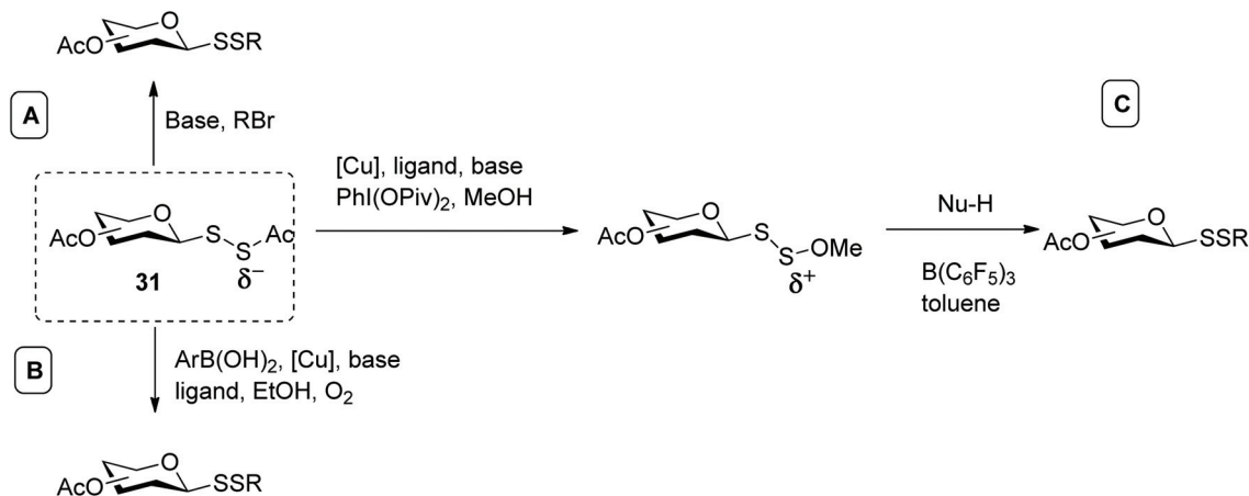
Scheme 11 Different methods to prepare disulfide-linked glycosides from glycosyl dithioperoxyester via : (A) A base-catalysed S N 2 process; (B) a copper-catalysed oxidative cross-coupling reaction; (C) an umpolung strategy.
