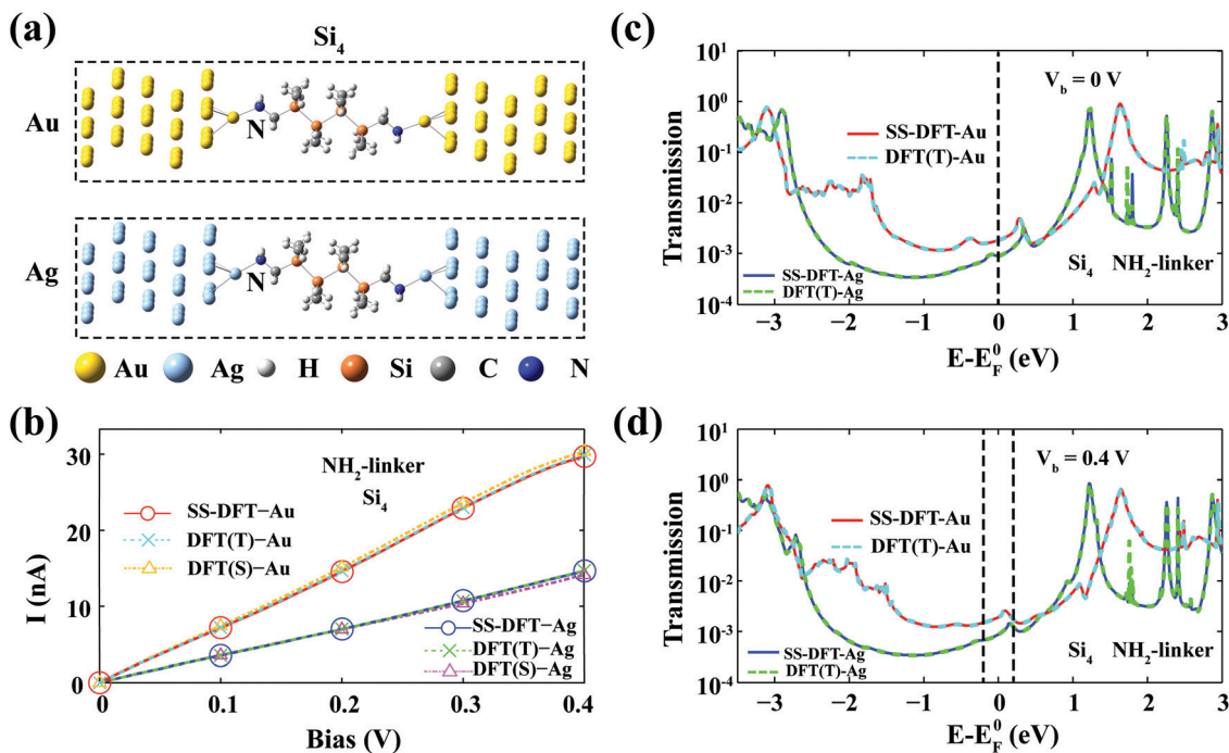
Fig. 1 Transport properties of the amine-terminated silane junctions \text{Si}_4\text{-NH}_2\text{-M} ( M = \text{Au} or \text{Ag} ). (b) The I - V curves of \text{Si}_4\text{-NH}_2\text{-M} calculated from SS-DFT and two DFT-based packages, TranSIESTA (DFT(T)) and SMEAGOL (DFT(S)). The three packages agree with each other remarkably well. (c) and (d) Transmission spectra obtained from SS-DFT and TranSIESTA are shown in (c) for V_b = 0 V and in (d) for V_b = 0.4 V. E_F^0 in (c) and (d) denotes the Fermi energy of the junction at zero bias.
