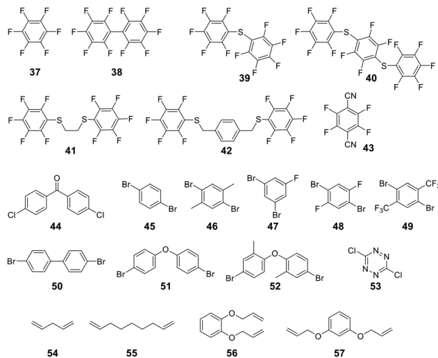
Fig. 3 Frequently used scaffold for thioether-based stapling by 1,4-disubstitution with perfluoro-scaffolds ( 37–42 ), Pd-mediated coupling with aryl dihalids ( 44–53 ) and thiol-ene reaction ( 54–57 ).
