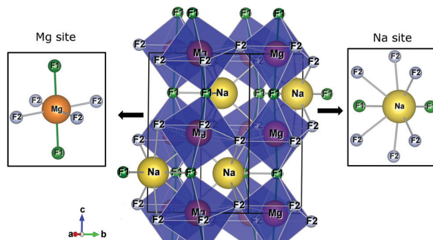
Fig. 1 The crystalline structure of \text{NaMgF}_3 in an orthorhombic lattice with space group Pbnm . Na and Mg sites are shown in detail.
