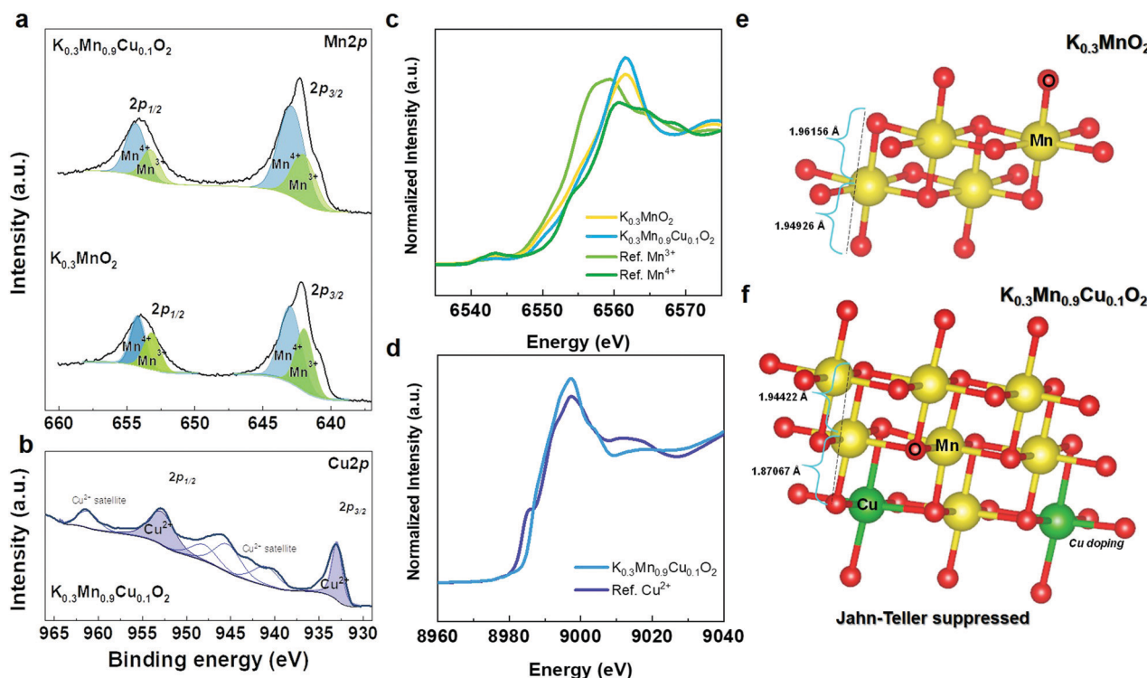
Fig. 4 (a) Mn 2P XPS spectra of KMO and KMCO and (b) Cu 2P XPS spectra of KMCO. (c) Mn K-edge XANES spectra of KMO and KMCO (ref. Mn 2 O 3 and MnO 2 ). (d) Cu K-edge XANES spectra of KMCO (ref. CuO). DFT structure model of Jahn teller distortion in (e) KMO and (f) KMCO.
