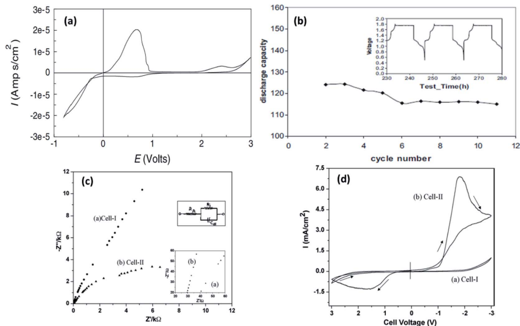
Fig. 10 Cyclic voltammetric curve recorded for Au/PVDF-Mg(AIEtBuCl 2 ) 2 -tetraglyme/Mg; (b) plot of discharge capacity vs. cycle number recorded at 80 °C for a battery with Mo 6 S 8 cathode, PVDF-Mg(AIEtBuCl 2 ) 2 -tetraglyme solid electrolyte, and AZ-31 Mg alloy anode (inset shows the voltage–time curve for the same battery). Reproduced from ref. 131 with permission, copyright 2003, Elsevier; (c) Nyquist plots and (d) cyclic voltammograms of cell 1 (SS|EMITf-PVDF-HFP|SS) and cell 2 (Mg|EMITf-PVDF-HFP|Mg) recorded at room temperature. Reproduced from ref. 136 with permission, copyright 2009, Wiley; inset in (c) shows the enlarged high-frequency region of the Nyquist plot.
