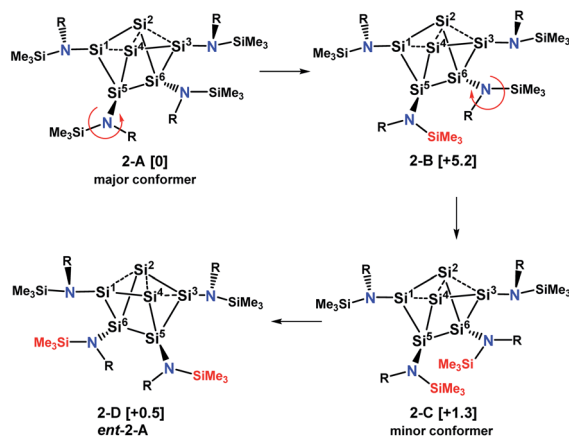
Scheme 5 Major and minor conformer and enantiomer of 2 in solution. Values in brackets are solvent corrected relative free energies \Delta G(298)_{\text{solv}} .
