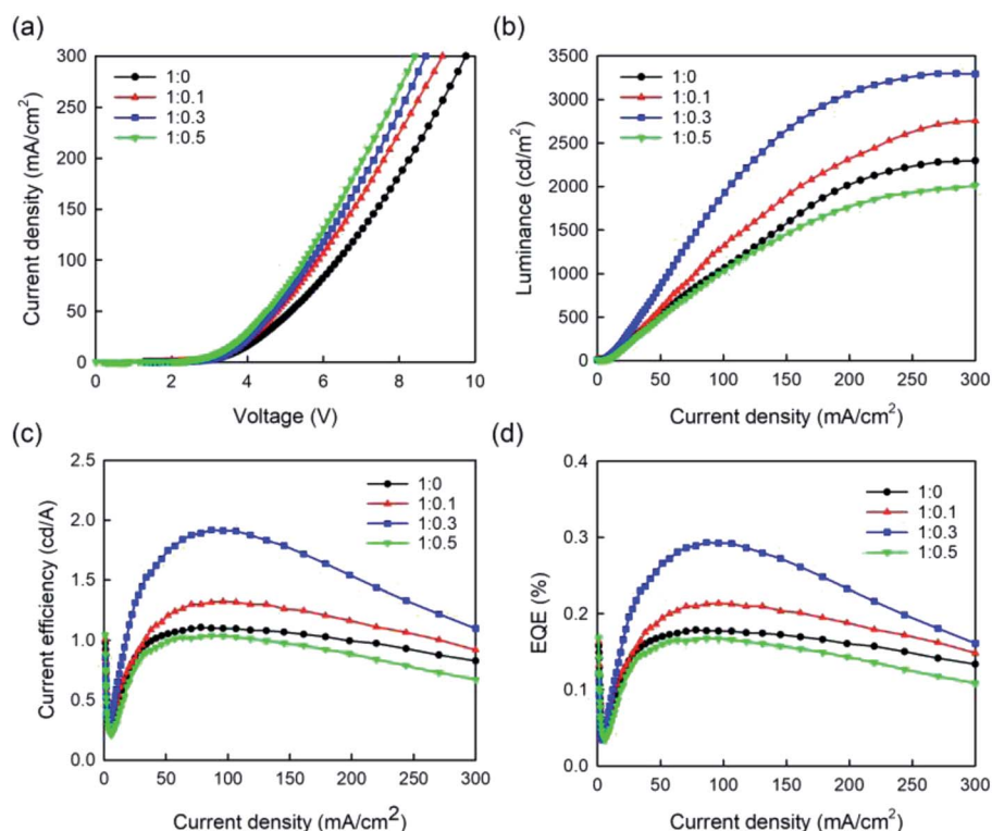
Fig. 6 (a) Current density vs. voltage, (b) luminance vs. current density, (c) current efficiency vs. current density, (d) external quantum efficiency vs. current density curves of PeLEDs with PEDOT:PSS HTLs doped with different GO content.
