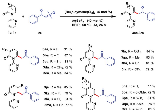
Scheme 2 Substrate scope of pyridions. a,b a Reaction conditions: compound 1a–1r (0.4 mmol), compound 2a (0.8 mmol), [\text{Ru}(p\text{-cymene})\text{Cl}_2]_2 (5 mol %), and \text{AgSbF}_6 (10 mol %) in HFIP (3 mL) at 60 °C, under Ar in 24 h. b Isolated yield.
