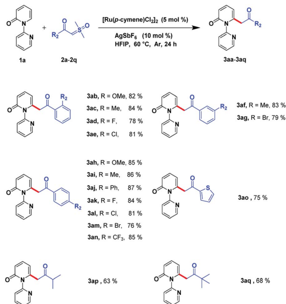
Scheme 3 Substrate scope of sulfoxonium ylides. a,b a Reaction conditions: compound 1a (0.4 mmol), compound 2a–2q (0.8 mmol), [\text{Ru}(p\text{-cymene})\text{Cl}_2]_2 (5 mol %), and \text{AgSbF}_6 (10 mol %) in HFIP (3 mL) at 60 °C, under Ar in 24 h. b Isolated yield.
