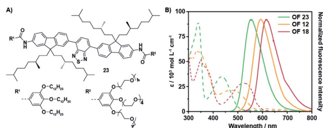
Fig. 2 Comparison of the optical properties between fluorene co-oligomers with and without the bridging vinyl moieties. (A) Molecular structure of OF 23. 38 (B) UV-Vis absorption spectra (dashed lines) and corresponding fluorescence spectra (solid lines) of OFs 12, 18 and 23 in THF ( c = 1.5 \times 10^{-5} M, \lambda_{\text{exc}} = 480, 510 and 430 nm, resp.).
