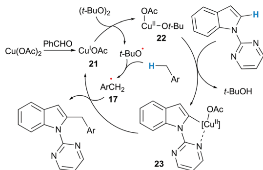
Scheme 12 C2-Benzylolation of 1-pyrimidyl-substituted indoles and proposed catalytic cycle.
