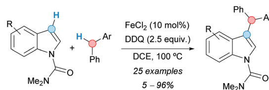
Scheme 13 C3-Benzylolation of 1- N,N -dimethylcarbamoyl indoles using a CDC approach.
