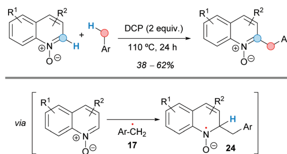
Scheme 14 C2-Benzylolation of quinoline- N -oxides using a CDC approach.
