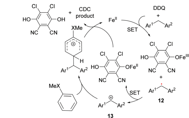
Scheme 5 CDC of substituted benzenes and diarylmethanes leading to triarylmethanes.
