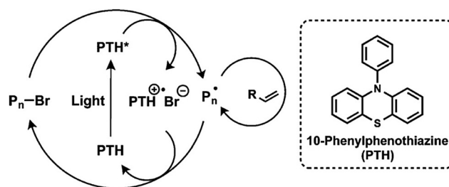
Fig. 1 Metal-free ATRP mediated by 10-phenylphenothiazine (PTH) as a photoredox catalyst. Adapted from ref. 26 with permission. Copyright (2014) American Chemical Society.
