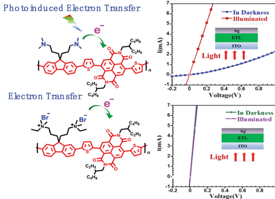
Fig. 33 Different doping processes of PNDIT-F3N and PNDIT-F3N-Br. Adapted from ref. 239 with permission. Copyright (2016) American Chemical Society.
