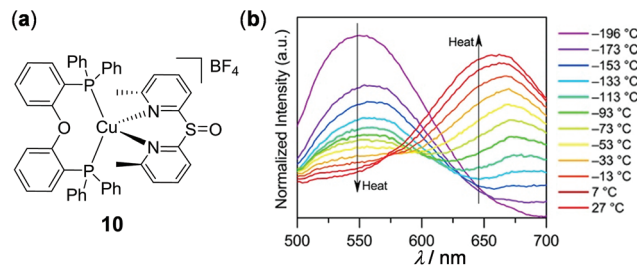
Fig. 9 (a) Molecular structure of Cu(I) complex 10 . (b) Normalized temperature-dependent emission spectral changes of 10 from -196 to 27 \text{ }^\circ\text{C} as thin films by drop-casting on quartz from MeOH solution ( \lambda_{\text{ex}} = 380 \text{ nm} ). Reprinted with permission from ref. 99. Copyright 2018 American Chemical Society.
