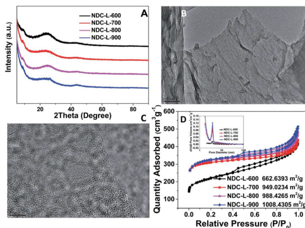
Fig. 1 (A) XRD pattern over the 2θ range of 5–90° of NDC-L-600, NDC-L-700, NDC-L-800, and NDC-L-900. (B) TEM and (C) HRTEM images of NDC-L-800. (D) N 2 adsorption–desorption isotherms of NDC-L-700, NDC-L-800, and NDC-L-900. The inset is pore-size distributions (PSDs) of the four samples.
