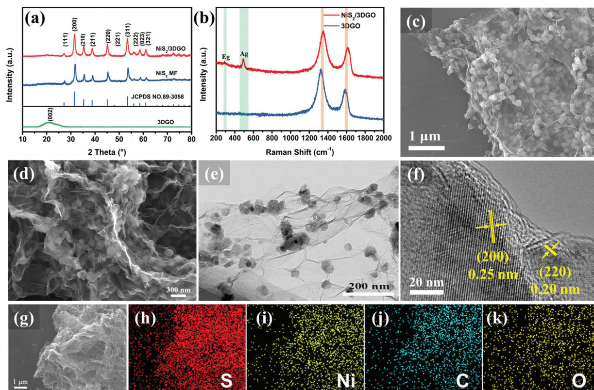
Fig. 2 (a) XRD comparison of \text{NiS}_2 /3DGO, \text{NiS}_2 MF and 3DGO; (b) Raman spectrum of \text{NiS}_2 /3DGO and 3DGO; (c and d) Representative SEM images of \text{NiS}_2 /3DGO; (e and f) TEM and HRTEM images of \text{NiS}_2 /3DGO; (g–k) SEM images and corresponding elemental mapping analysis of \text{NiS}_2 /3DGO.
