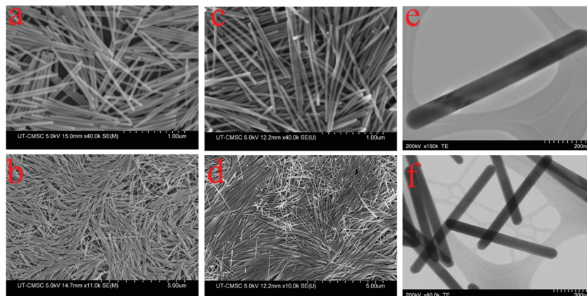
Fig. 1 SEM images of Te NWs obtained from TeO 2 with ethylene glycol at 120 °C (a) and (b) 0.1 g PVP and 0.75 mL ascorbic acid (c) and (d) 0.2 g PVP and 1.5 mL ascorbic acid and (e) and (f) STEM images of Te NWs obtained from 0.1 g PVP and 0.75 mL ascorbic acid.
