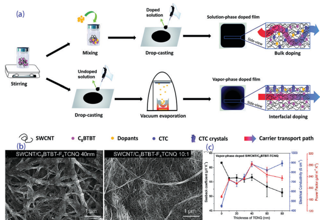
Fig. 11 (a) Fabrication processes of the composite films by bulk doping or interfacial doping, (b) SEM pictures of an SWCNT/C 8 BTBT-F 4 TCNQ film obtained with a vapor-phase process and an SWCNT/C 8 BTBT-F 4 TCNQ film obtained with a solution-phase process, and (c) the transport properties of vapor-phase doped SWCNT/C 8 BTBT-TCNQ with different thicknesses of TCNQ. 145
