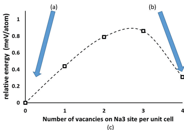
Fig. 2 The two lowest energy configurations for \text{Na}_{11}\text{Sn}_2\text{PS}_{12} : (a) the lowest energy configuration containing 8 vacancies on Na2 (32g) sites, (b) the second-lowest energy configuration with the Na/vacancy distribution previously reported by Yu et al. 47 containing four vacancies on Na2 (32g) sites and four on Na3 (16d) sites. Grey (brown) tetrahedra represent \text{SnS}_4 ( \text{PS}_4 ), green spheres occupied Na sites, while Na2 (Na3) vacancies are marked in red (magenta). (c) Energy profile for the lowest energy interconversion between these two configurations.
