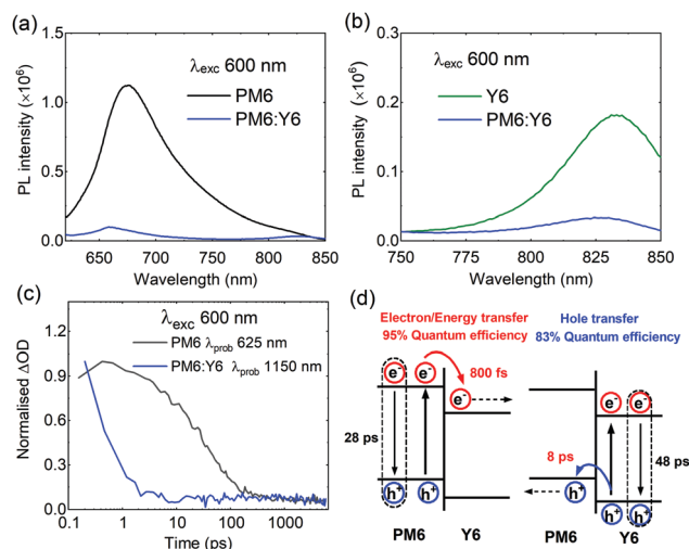
Fig. 2 (a) Steady-state PL spectra of films excited on 600 nm for electron transfer from PM6 and (b) hole transfer from Y6. (c) Transient absorption decay dynamics for neat PM6 and PM6:Y6 blend films. (d) A schematic showing exciton decay and charge/energy transfer processes.
