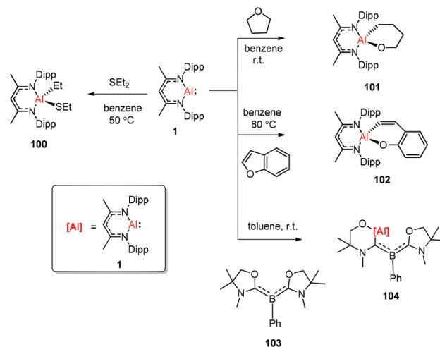
Scheme 25 \text{C-O} and \text{C-S} bond activation, respectively, by the aluminum(i) compound.
