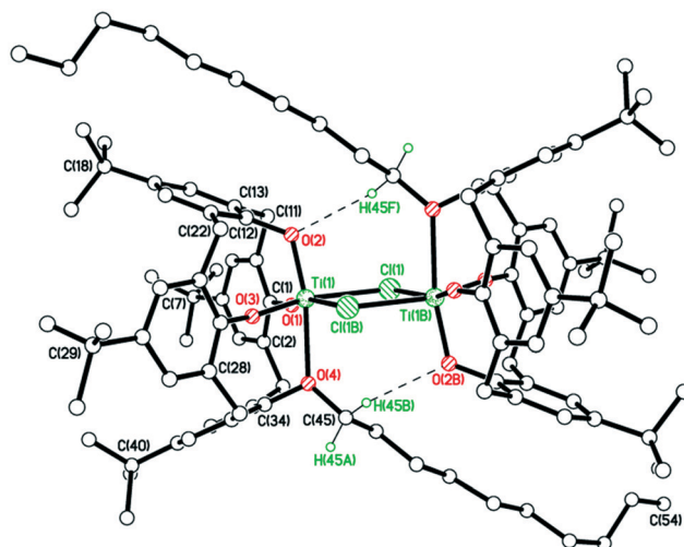
Fig. 2 Molecular structure of \{[\text{Ti}(\text{L}(\text{O})_3(\text{OR}))_2](\mu\text{-Cl})_2\}\cdot 4\text{MeCN} ( R = n -decyl (4-6MeCN)) (most H atoms and solvent molecules are omitted for clarity). Selected bond lengths (Å) and angles ( ^\circ ): Ti(1)–Cl(1) 2.4454(12), Ti(1)–Cl(1B) 2.5257(10), Ti(1)–O(1) 1.794(2), Ti(1)–O(2) 1.825(3), Ti(1)–O(3) 1.792(3), Ti(1)–O(4) 2.390(3); Ti(1)–O(1)–C(1) 161.5(2), Ti(1)–O(2)–C(12) 121.9(2), Ti(1)–O(3)–C(23) 158.1(3), Ti(1)–O(4)–C(34) 115.0(2), Cl(1)–Ti(1)–Cl(1B) 77.04(4).
