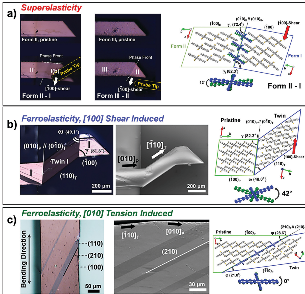
Fig. 15 (a) Superelasticity of #13 crystal in Fig. 2 based on [100] shear induced Form II–I and Form III–II transition. (b) Ferroelasticity of #13 crystal based on [100] shear and (c) [010] tension induced. Adapted with permission from ref. 57, copyright 2020 John Wiley & Sons, Inc.
