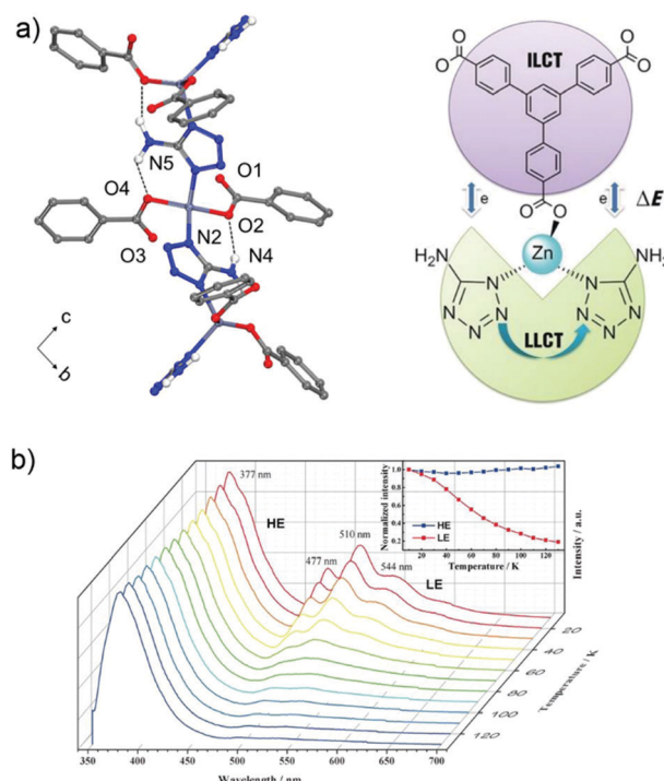
Fig. 3 (a) 1D zigzag chain in [(CH 3 ) 2 NH 2 ][Zn(btbt) 2/3 (atz)] with N-H...O hydrogen bonds (top). The Dexter energy transfer (DET) mechanism in a dual emissive system (down). (b) Emission spectra of [(CH 3 ) 2 NH 2 ][Zn(btbt) 2/3 (atz)] recorded between 10 and 130 K (λ ex = 330 nm). Reproduced from ref. 60 with permission of John Wiley & Sons, Ltd, copyright 2016.
