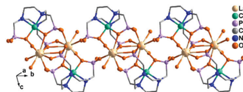
Fig. 5 Chain structure of 36 . All H atoms are omitted for clarity. Adapted from ref. 32.
