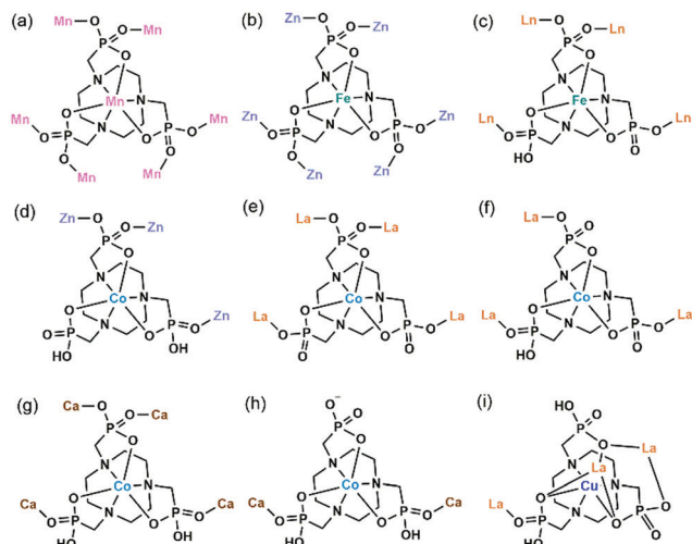
Scheme 5 Coordination modes of M(\text{notpH}_x) metallogligands.
