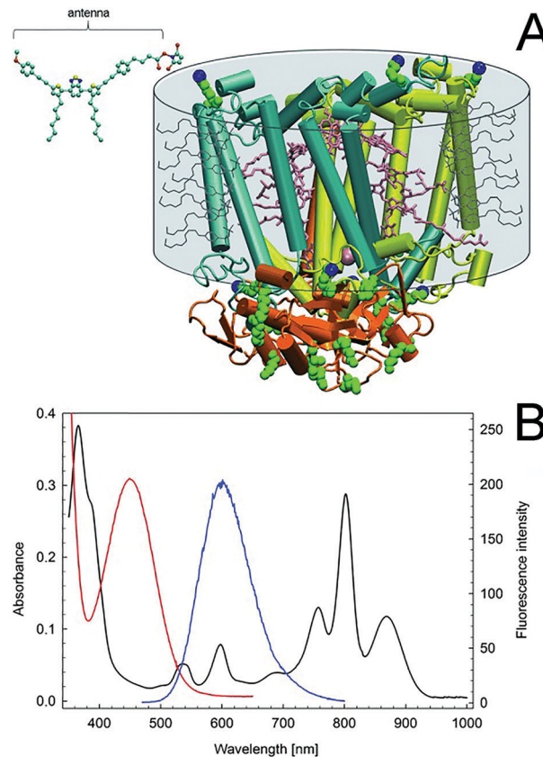
Fig. 9 (A) Crystallographic structure of the Rhodobacter sphaeroides R26 reaction center. The ubiquinone-10 molecules ( Q_A , Q_B ), two bacterio-pherophytins, and four bacteriochlorophylls are in pink. Lysines are van der Waals green spheres. The terminal N_\epsilon lysine targets of bioconjugation are in blue. The detergent toroid surrounding the hydrophobic portion of the protein is shown as a grey cylinder, including the detergent molecules (not to scale). The structure of the activated organic fluorophore antenna is shown in the upper left corner (C, cyan; N, blue; O, red; and S, yellow). The antenna and the RC structures are to scale. (B) Absorption spectra of the RC (black) and the artificial antenna (red). Fluorescence spectrum of the antenna (blue). Adapted with permission from F. Milano, R. R. Tangorra, O. Hassan Omar, R. Ragni, A. Operamolla, A. Agostiano, G. M. Farinola and M. Trotta, Enhancing the Light Harvesting Capability of a Photosynthetic Reaction Center by a Tailored Molecular Fluorophore, Angew. Chem., Int. Ed. , 2012, 51 , 11019–11023. Copyright 2012 Wiley-VCH Verlag GmbH & Co. KGaA.
