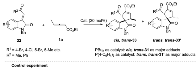
Scheme 10 Phosphine-catalysed highly diastereoselective (3+2) annulations of isatin derived electron-deficient alkenes.
