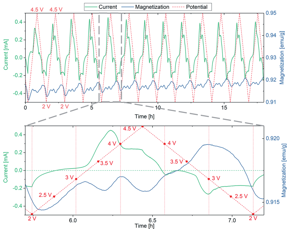
Fig. 1 First 13 cycles of the FeF 3 ·3H 2 O/Li insertion reaction (top) with a more detailed view of the 5 th cycle (bottom). CV/SQUID measurements showing the evolution of magnetization with current and potential. The sweep rate was 1 mV s -1 . The horizontal dashed green line in the bottom panel represents the zero line of current, while the vertical red dotted lines denote the potential at the respective time. Corresponding cyclic voltammograms can be found in the ESI (Fig. S2†).
