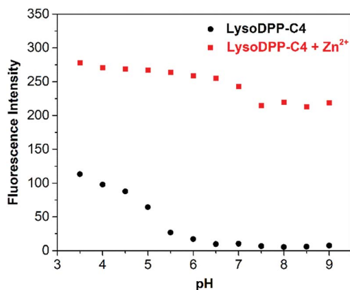
Fig. 2 Fluorescence intensity of LysoDPP-C4 ( 1 \mu\text{M} ) and its zinc complex in solutions of varying pH (0.05 M NaCl aqueous solution). \lambda_{\text{ex}} = 430 \text{ nm} / \lambda_{\text{em}} = 515 \text{ nm} .
