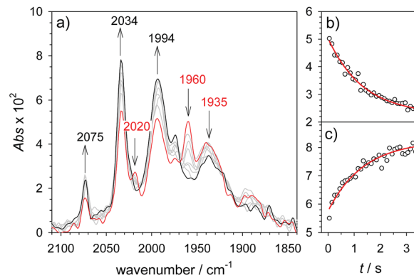
Fig. 4 Rapid scan FTIR spectra in acetonitrile between 50 ms (—) and 3 s (---) after mixing of 1H + (1.3 mM 1 , 2.6 mM Cl 2 BSA) with cobaltocene (20 mM) (a) and kinetic traces (○) with exponential fits (—) monitoring decay of 1H at 1960 cm −1 (b) and formation of 1 at 2034 cm −1 (c).
