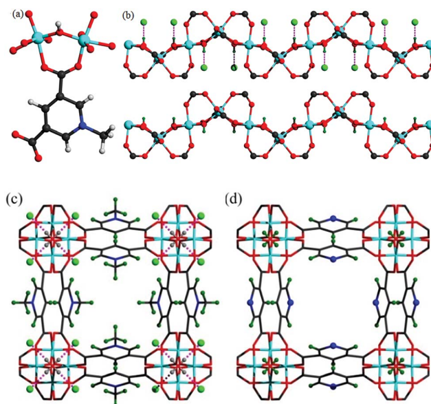
Fig. 1 (a) View of the coordination environment for ligand L − and the Al(III) centre. (b) View of the corner-sharing octahedral chain of [AlO 4 (OH) 2 ] ∞ . The μ 2 -(OH) groups form hydrogen bond to Cl − . Views of (c) MFM-305-CH 3 and of (d) MFM-305. The pore size is ~4.6 × 4.6 Å for MFM-305-CH 3 and ~5.6 × 5.6 Å for MFM-305 taking into consideration van der Waals radii. The methyl groups (olive) and chloride ions (green) in MFM-305-CH 3 ; N atoms (blue) and hydroxyl group (olive) in MFM-305.
