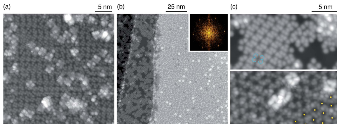
Fig. 6 STM images of (a) Tb(tbuc-Pc) 2 embedded in a tbuc-2H-Pc layer after RT deposition of Tb on tbuc-2H-Pc molecules; (b) after annealing at 570 K for 30 min. Left terraces: mainly free-base molecules, right terrace: large-scale ordered islands of Tb(tbuc-Pc) 2 ; (inset) FFT obtained from a region exclusively covered by Tb(tbuc-Pc) 2 . (c) High-resolution STM images of different regions of the annealed sample. Top: tbuc-2H-Pc molecules; the cyan circles highlight a single tbuc-2H-Pc molecule in the assembly. Bottom: Tb(tbuc-Pc) 2 molecules; the yellow dots in the lower-right corner indicate the center of the molecules and serve as a guide to the eye. Brighter molecules are second-layer Tb(tbuc-Pc) 2 (1.8 ML tbuc-2H-Pc/Ag(111) + 0.6 ML Tb; V_t = -2.0 V, I_t = 50 pA, T = 5 K).
