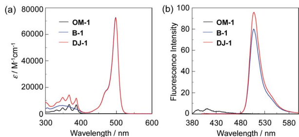
Fig. 2 (a) Photoabsorption and (b) fluorescence ( \lambda^{\text{ex}} = 366 nm for OM-1 and 367 nm for B-1 and DJ-1 , respectively) spectra of OM-1 ( c = 2.0 \times 10^{-5} M), B-1 ( c = 4.0 \times 10^{-6} M), and DJ-1 ( c = 4.0 \times 10^{-6} M) in acetonitrile.
