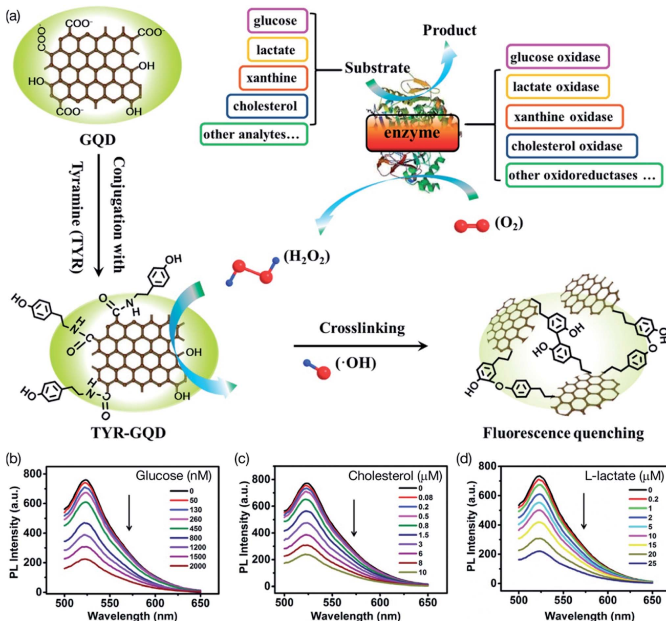
Fig. 32 (a) Schematic illustration of fluorescence detection scheme using tyramine-functionalized GQDs (TYR-GQDs). (b) Photoluminescence (PL) spectra of 0.1 mg mL -1 TYR-GQD in PBS (pH 7.0) containing 2.5 \mu\text{M} glucose oxidase and at different concentrations of glucose. (c) PL spectra of spectra of 0.1 mg mL -1 TYR-GQD in PBS (pH 7.0) containing 10 \mu\text{M} cholesterol oxidase and at different concentrations of cholesterol. (d) PL spectra of 0.1 mg mL -1 TYR-GQD in PBS (pH 7.0) containing 5 \mu\text{M} lactate oxidase and at different concentrations of L-lactate. [Reprinted with permission from ref. 670, N. Li, A. Than, X. Wang, S. Xu, L. Sun, H. Duan, C. Xu and P. Chen, Ultrasensitive Profiling of Metabolites Using Tyramine-Functionalized Graphene Quantum Dots , ACS Nano , 2016, 10, 3622–3629. Copyright© American Chemical Society.]
