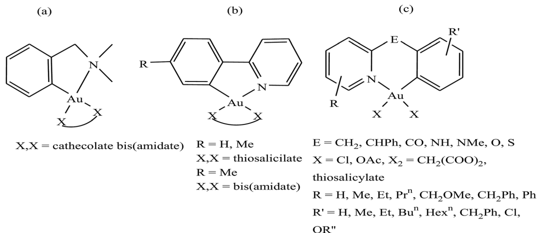
Fig. 23 Chemical structure of a series of a series of cycloaurated complexes (a) [Au(dmamp)(X-X)], (b) [Au(R-C N )(X-X)] and (c) [Au(R-N E C-R')(X-X)].
