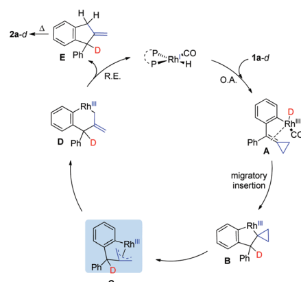
Scheme 4 A plausible reaction mechanism.
