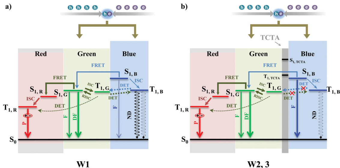
Fig. 6 Working mechanisms of devices W1 (a) and W2 and W3 (b). Here, S_{1,B} , S_{1,G} , and S_{1,R} are the singlet energy levels of TPB-AC, CP-BP-PXZ, and Ir(dmppr-mp) _2 (divm), respectively. T_{1,B} , T_{1,G} , and T_{1,R} are the triplet energy levels of TPB-AC, CP-BP-PXZ, and Ir(dmppr-mp) _2 (divm), respectively. FRET and DET are the Förster and Dexter energy transfer, respectively. P, F, DF, and ND are the phosphorescence, fluorescence, delayed fluorescence, and non-radiative decay, respectively. ISC and RISC are the intersystem crossing and the reverse intersystem crossing, respectively.
