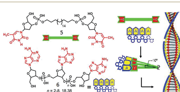
Fig. 2 (left) Structure of thymidine-appended bolaamphiphile and adenylic acid oligomers. (right) Proposed mechanism of templated assembly. Adapted and modified with permission from ref. 23. Copyright 2003, Wiley-VCH.
